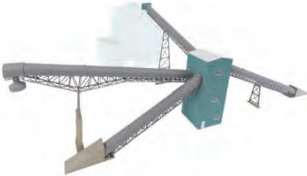
933-4171 Coal Conveyor with Transfer House Kit
