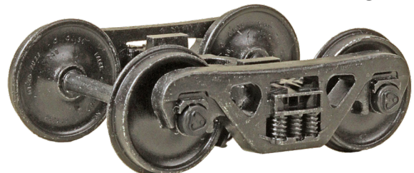
#754 A.S.F 100-ton Roller Bearing
