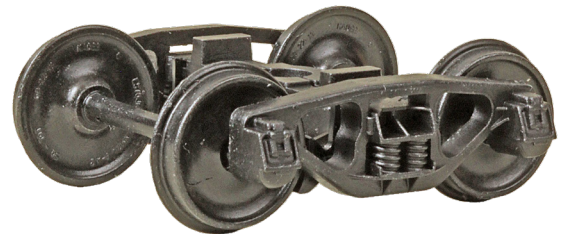
#751 AAR Bettendorf Style
